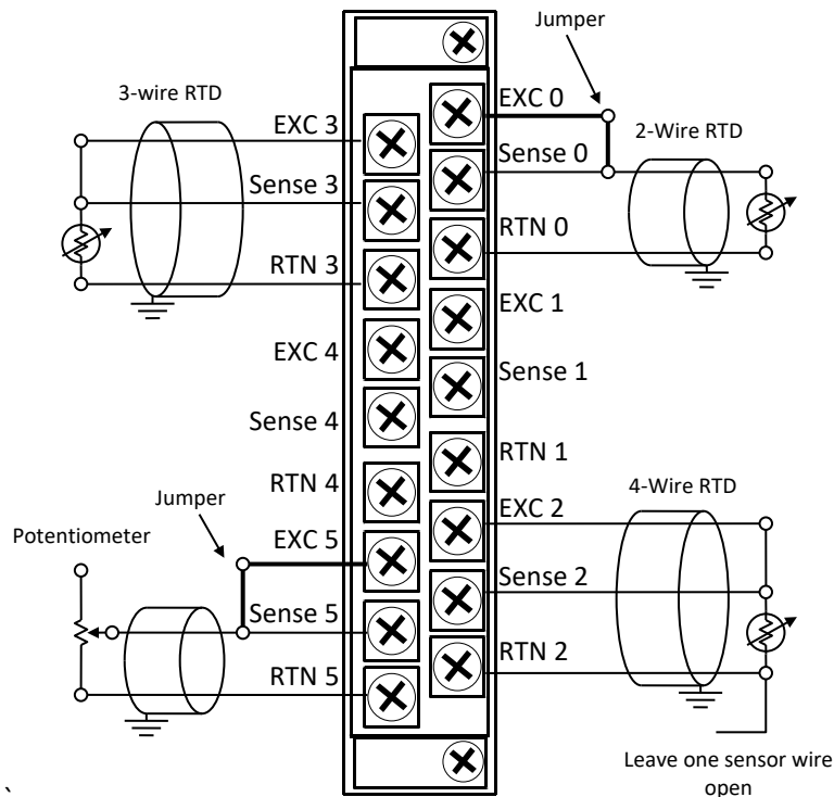
Figure 2-1. Wiring Diagram
