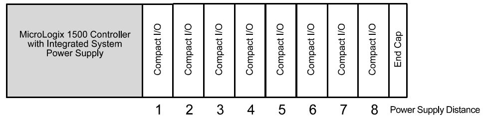
Figure 2-1. Power Supply Distance
