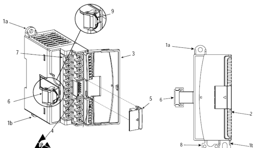
Figure 1-1. Hardware Features
