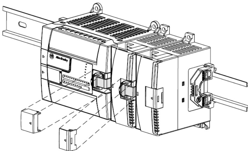
Figure 2-4. Expansion IO Attachment
