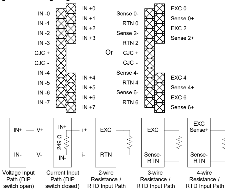
Figure 2-1. Wiring Diagram
