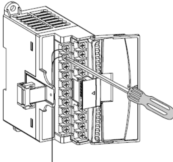
Figure 2-6. Wiring
