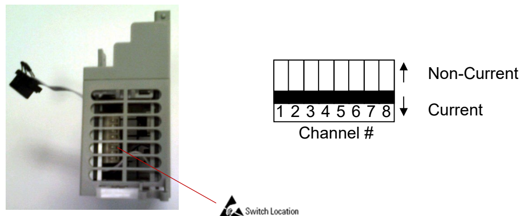
Figure 3-1. Dip-Switch Settings
