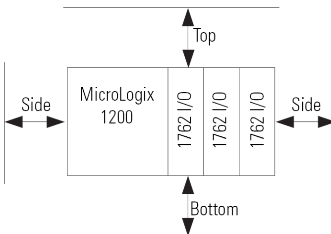
Figure 2-1. Minimum Spacing
