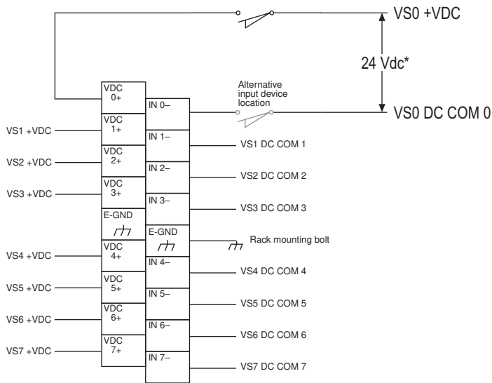
1746sc-IB8I Isolated-Circuit 24 Vdc Inputs (8)
