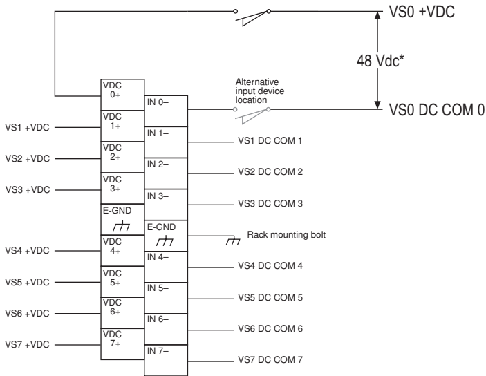
1746sc-IC8I Isolated-Circuit 48 Vdc Inputs (8)
